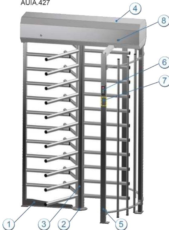
Sesame-A Basic AUJA.427
